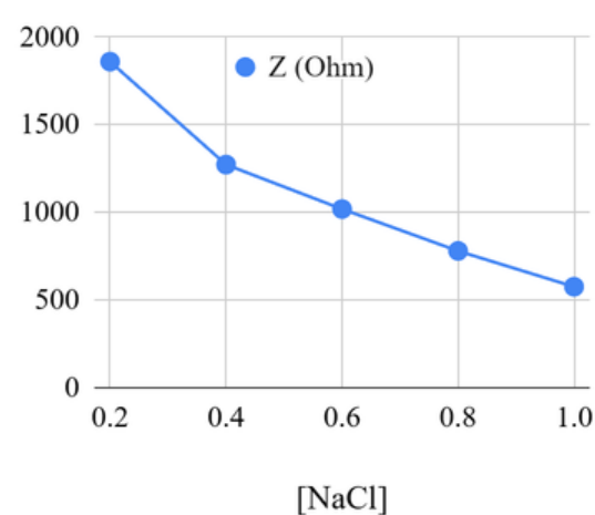
Salt Addition vs Resistance
